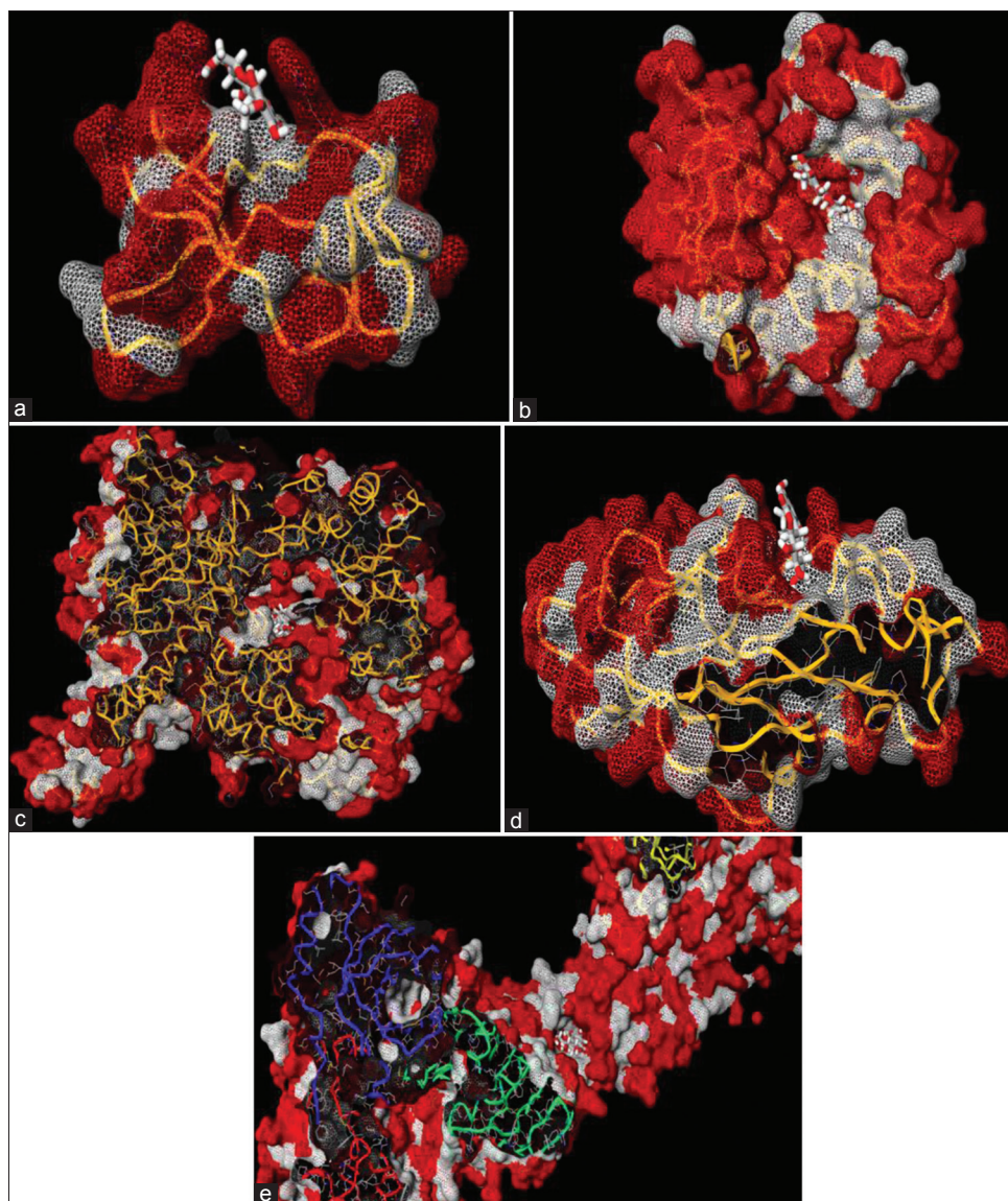
Figure 2: Host targets for buffer ground electrolyte (a) purine nucleoside phosphorylase, (b) carbonic anhydrase XIV, (c) ADAM17, (d) xanthine oxidoreductase, (e) Type 1 fimbriae D-mannose-specific adhesion
